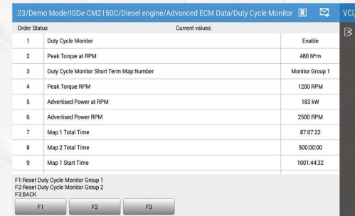
Duty cycle monitor
